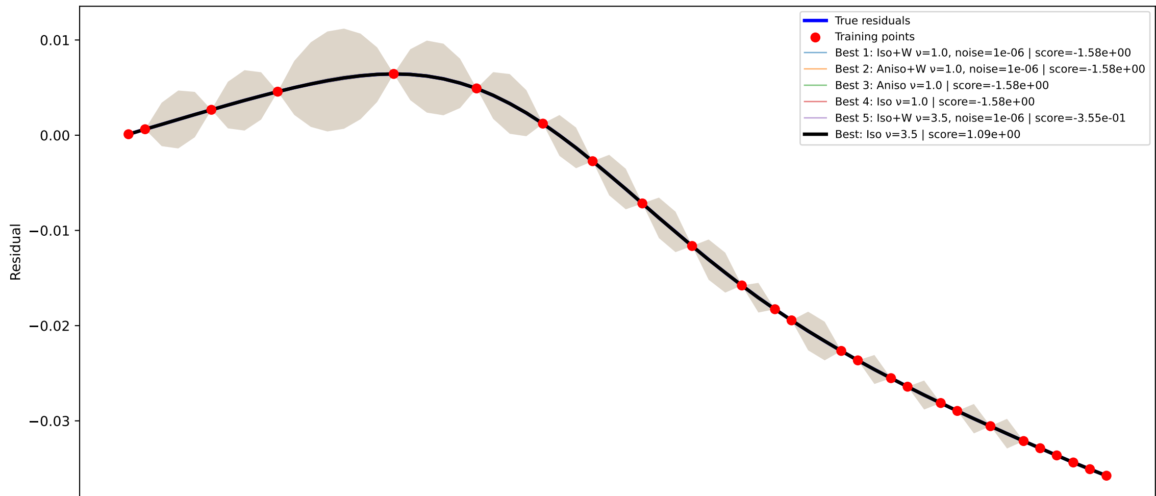
GPR kernel comparison node=1 RMSE=3.094e-06, train RMSE=7.024e-09
